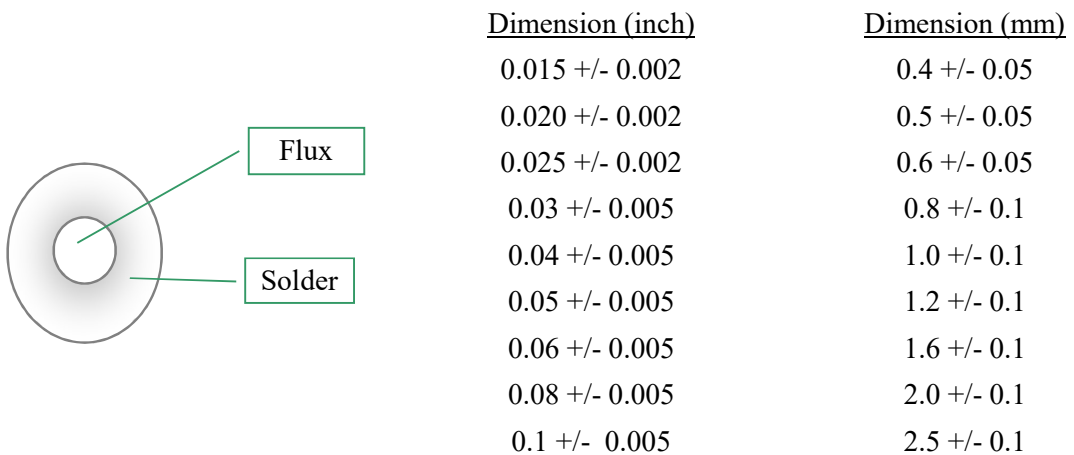
Figure (1) Wire Cross Section
